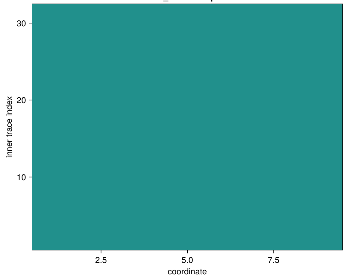
s_{\text{ref}} heatmap
