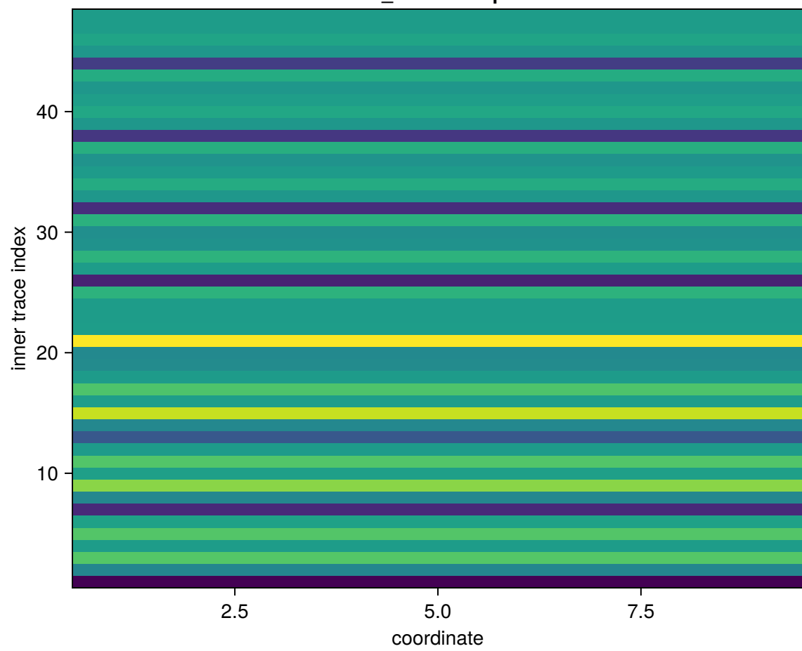
x_{\text{ref}} heatmap
